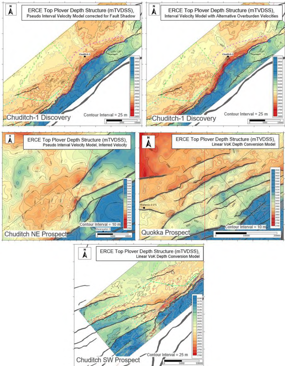
Figure 3.3: ERCE Top Plover depth-converted grids in mTVDSS.
