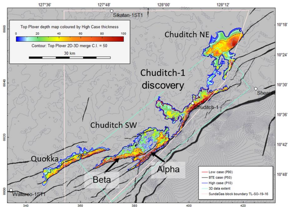
Figure 3.1: SundaGas' Merged 3D final PSDM / 2D Top Plover depth structure map
