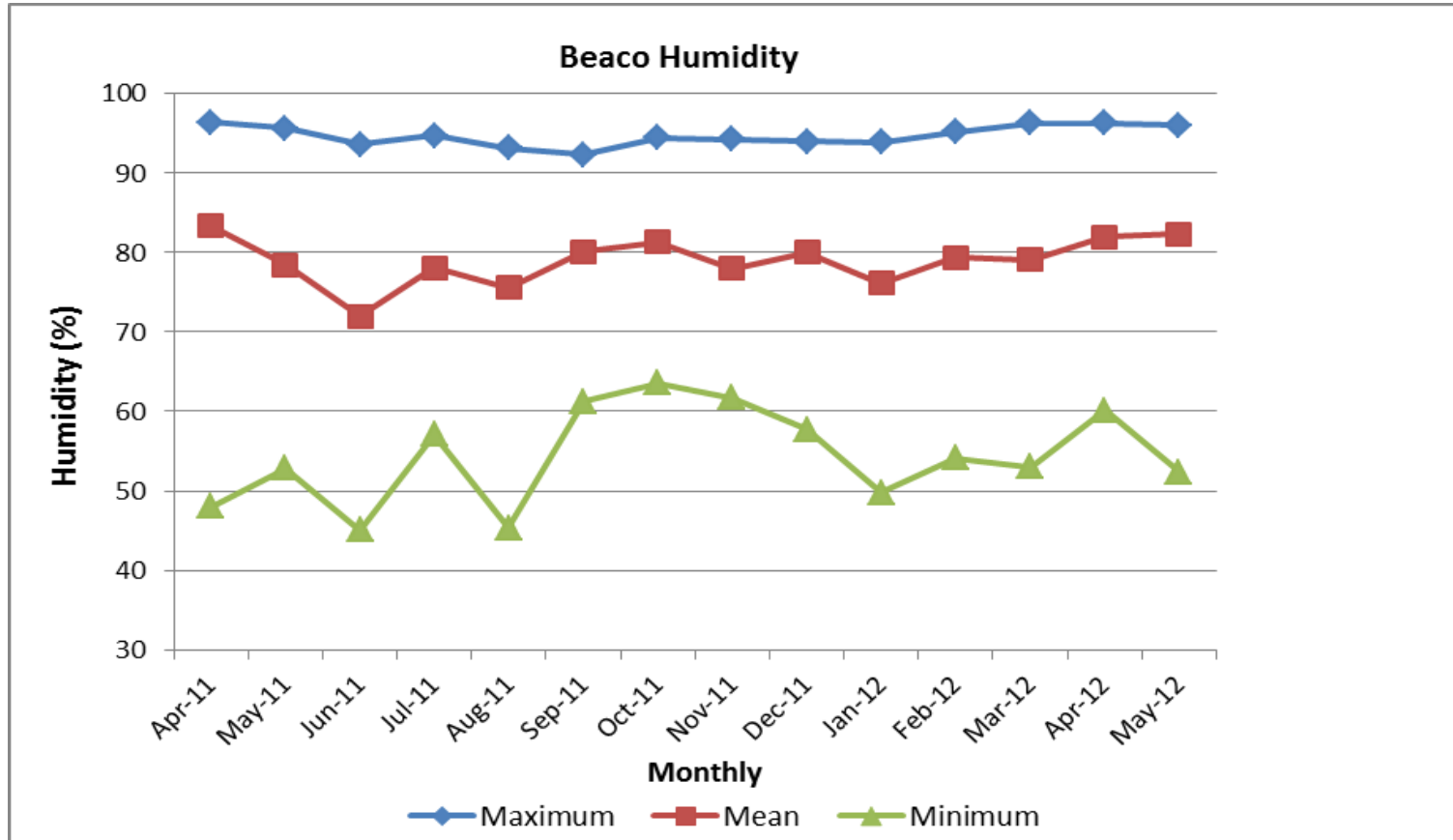
Figure 14- Humidity Level in Beaço
