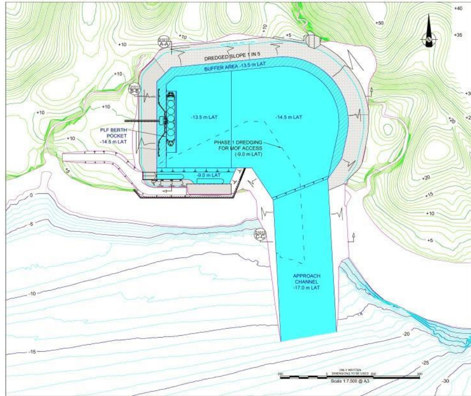
Figure 5 – Detailed Drawing of Marine Facility (LNG Port)
