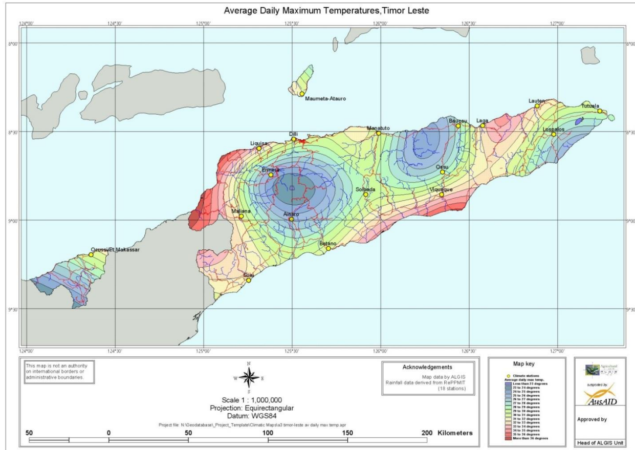
Figure 8 - Daily Maximum Temperature of Timor-Leste
