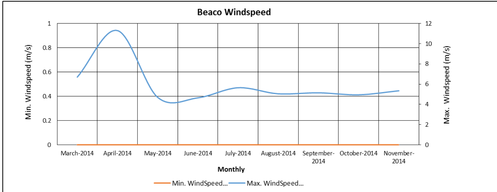
Figure 17 - Beaço Wind Speed Recorded in 2014
