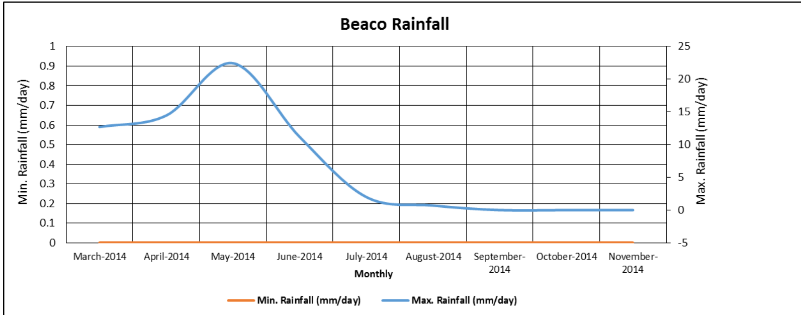
Figure 13 - Maximum and Minimum of Beaco Rainfall Rate
