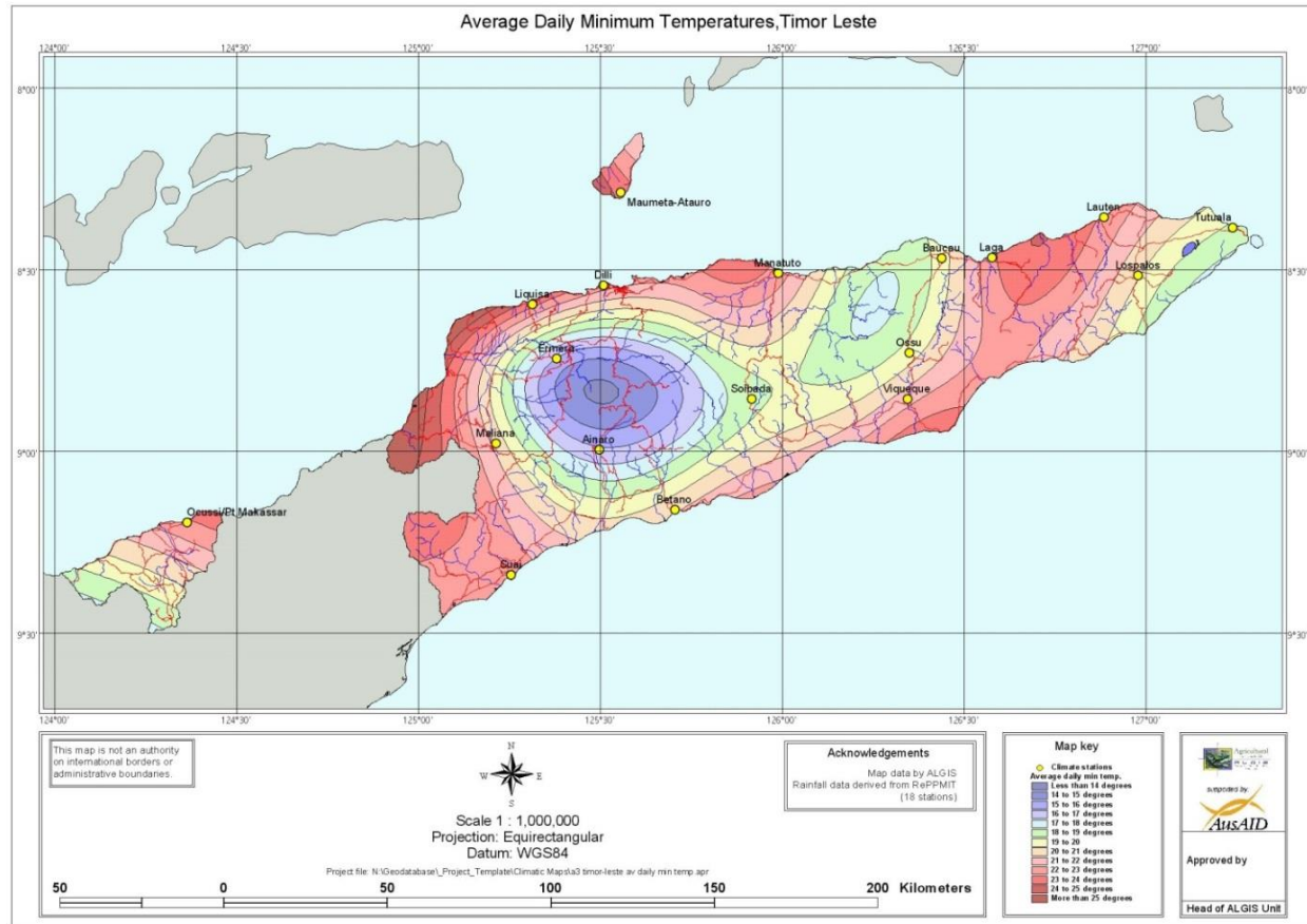
Figure 9 - Daily Minimum Temperature of Timor-Leste
