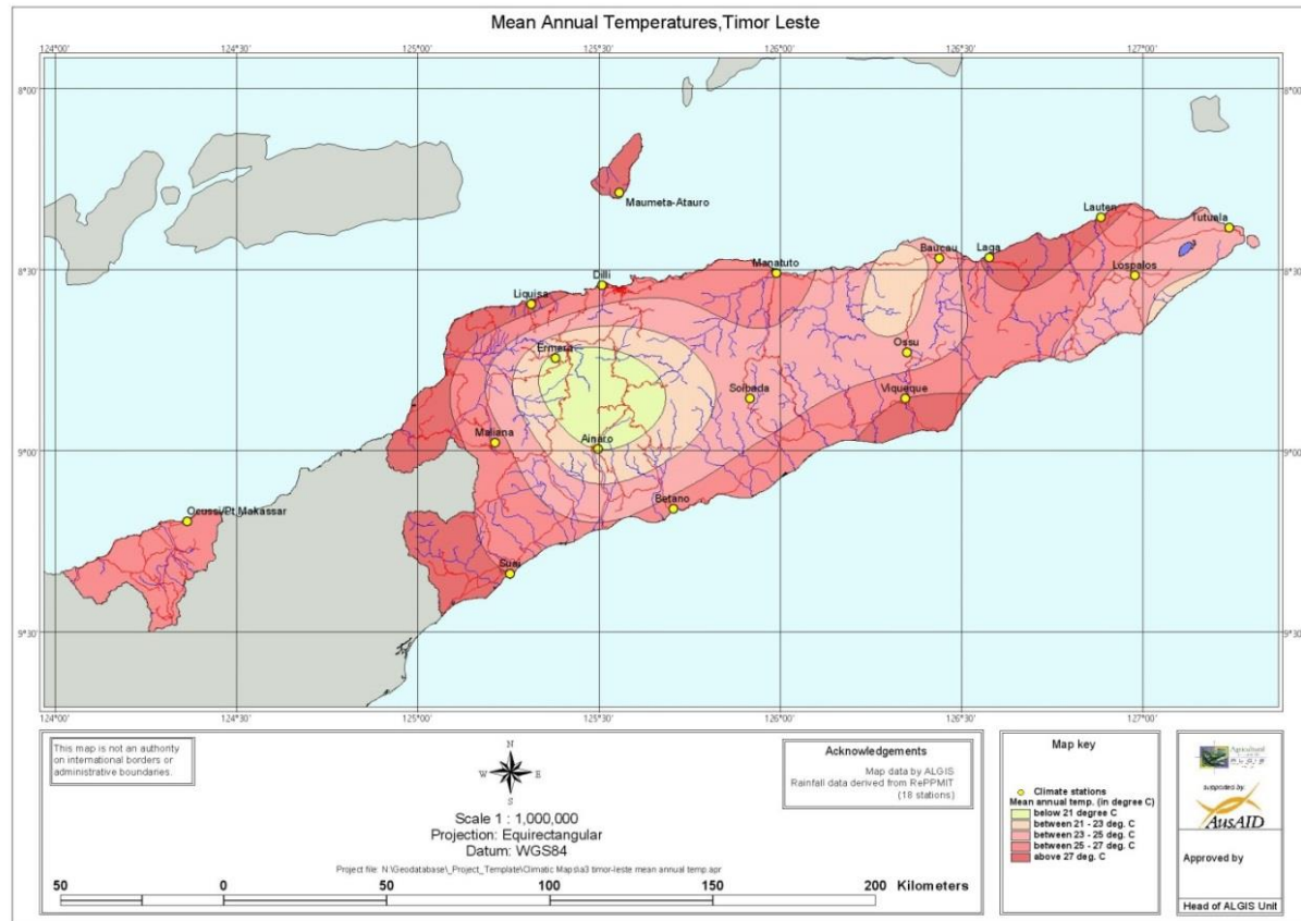
Figure 10 - Mean annual Temperature of Timor-Leste
