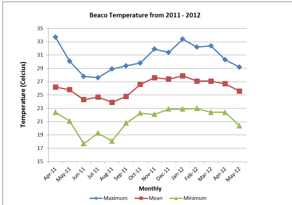
Figure 7 – Beaço Temperature Recorded from 2011 - 2012
