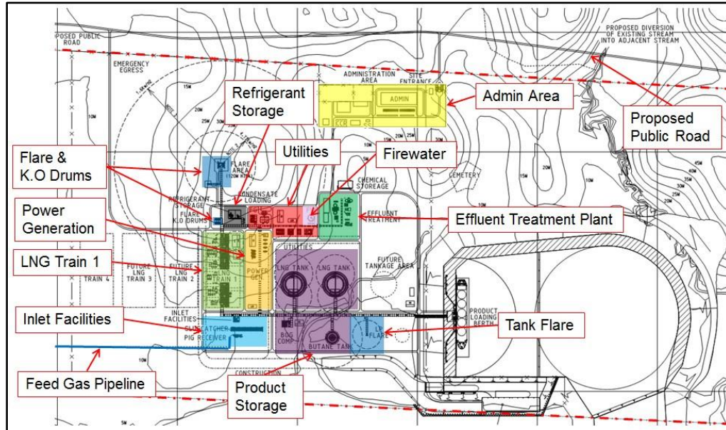
Figure 4 - Major Units of LNG Plant (Source: TIMOR GAP-LNG Plant Pre FEED Study, 2016)
