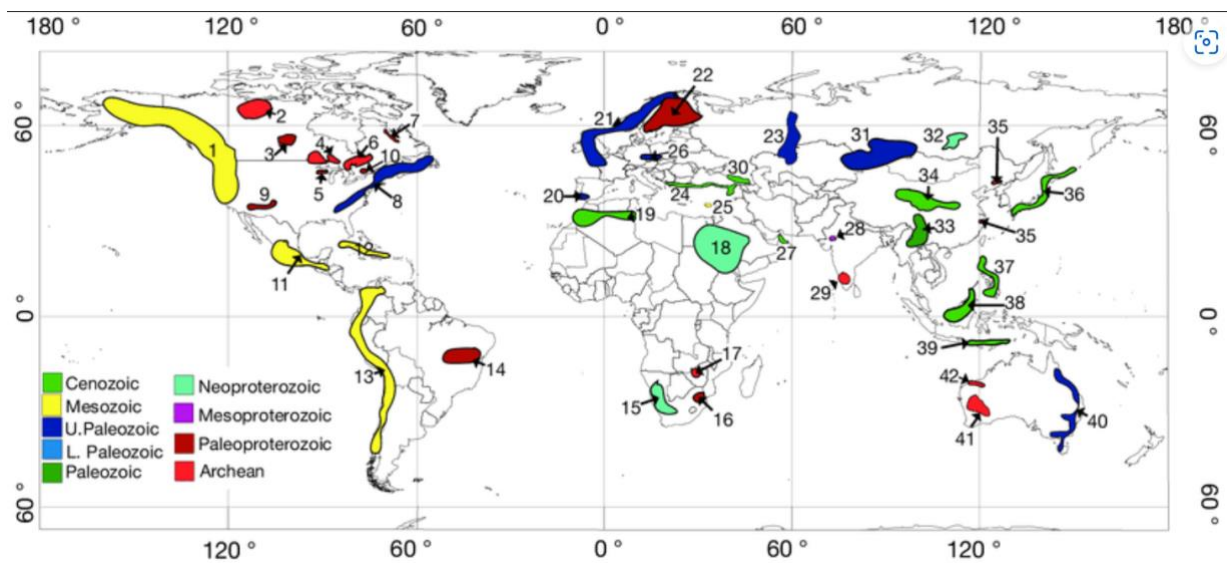
Figure 4: Worldwide locations of principal orogens containing VMS deposits
